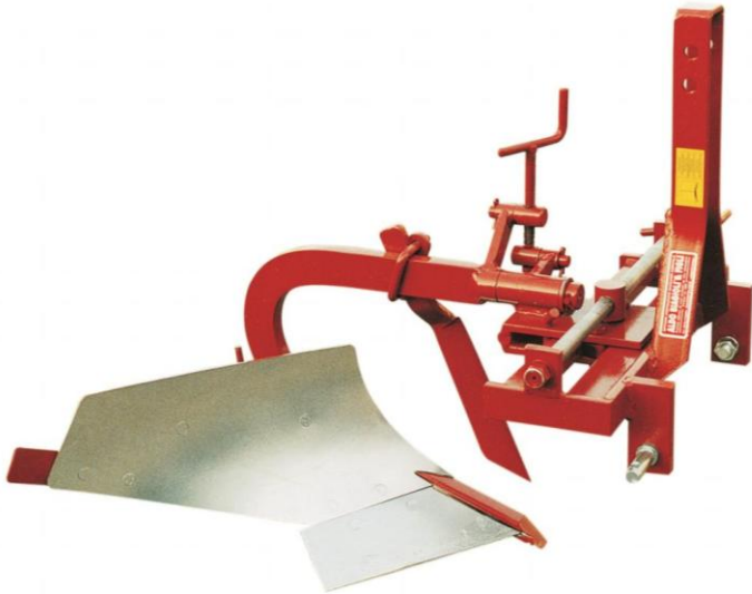
Aratro monovomere MDS con attacco a spostamento a vite Charrue monosoc MDS soc à carrelet - déplacement à vis Single furrow chisel plough MDS - displacement by screw
